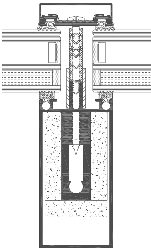
MC FIRE transom cross section (MC534)
