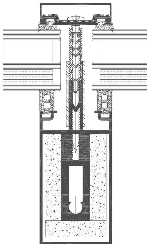
MC FIRE mullion cross section (MC014)
